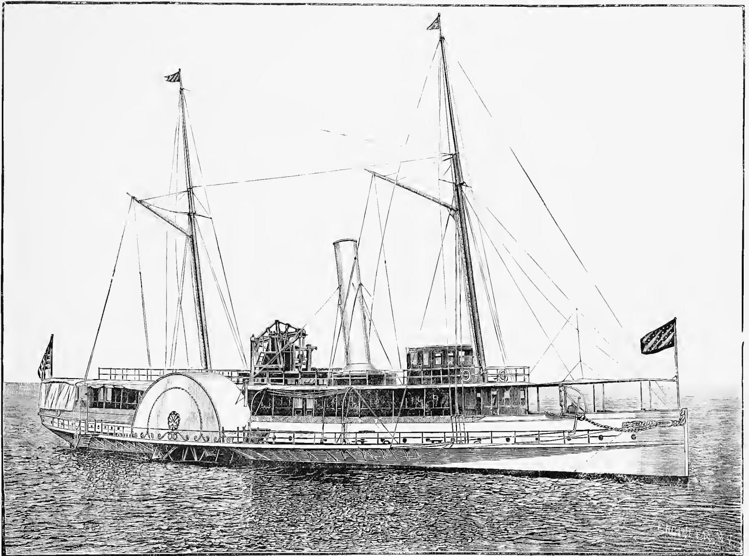
A. VAN SANTVOORD'S WOODEN STEAM YACHT CLERMONT.—Machinery by the W. & A. Fletcher Co., Hoboken, N. J.
